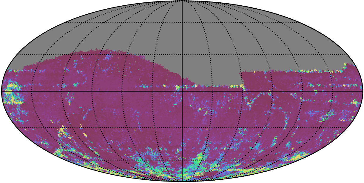
too_combined_no_gw_s10.0_v3.4_10yrs All sky z band: 75th Percentile Intranight Timespan
