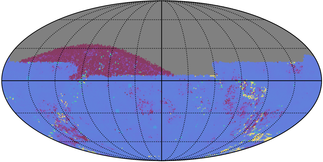
too_combined_no_gw_s10.0_v3.4_10yrs All sky ug bands: 75th Percentile Intranight Timespan
