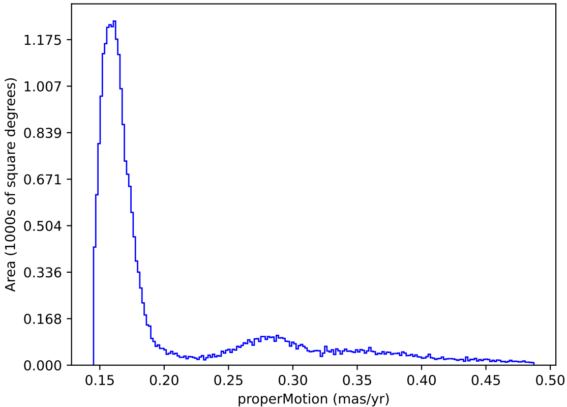
too_combined_no_gw_s10.0_v3.4_10yrs : properMotion
