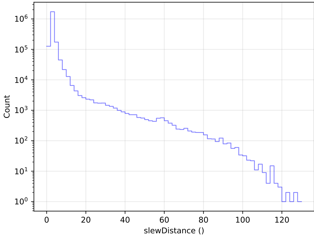
too_combined_no_gw_s10.0_v3.4_10yrs All visits: Slew Distance Histogram
