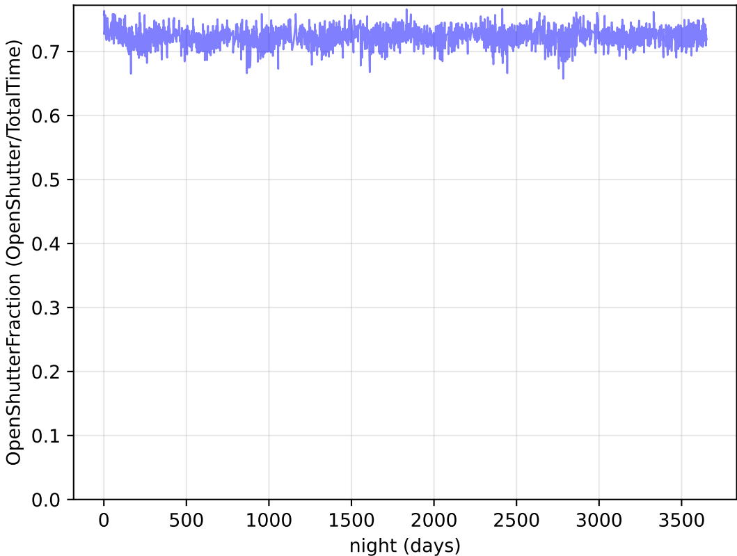
too_combined_no_gw_s10.0_v3.4_10yrs : OpenShutterFraction
