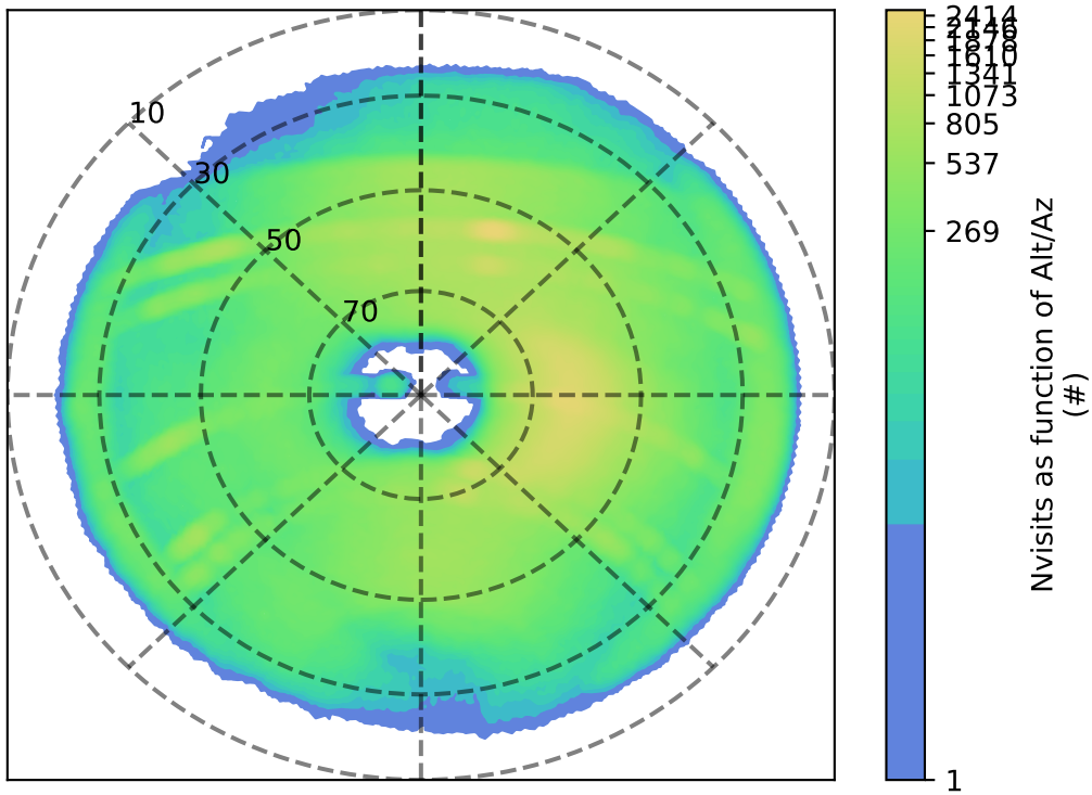
too_combined_no_gw_s10.0_v3.4_10yrs z: Nvisits as function of Alt/Az
