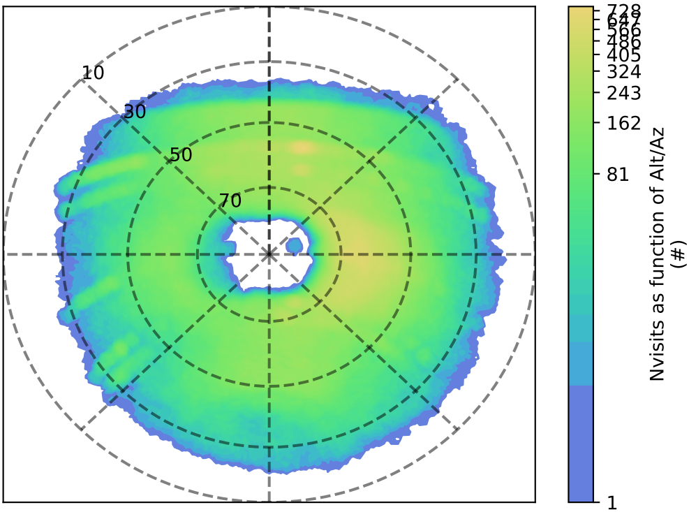
too_combined_no_gw_s10.0_v3.4_10yrs u: Nvisits as function of Alt/Az
