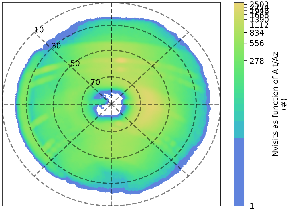
too_combined_no_gw_s10.0_v3.4_10yrs r: Nvisits as function of Alt/Az
