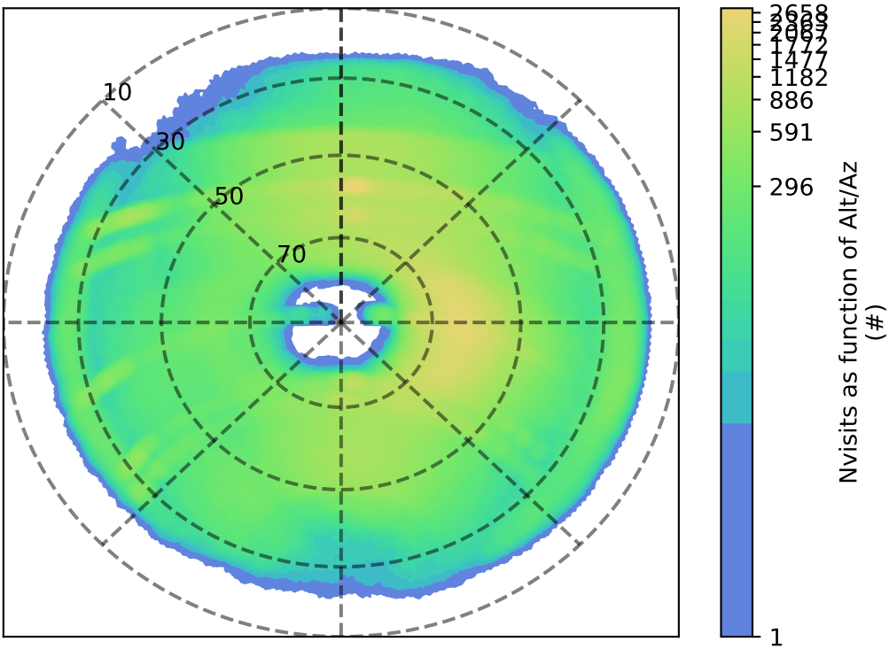
too_combined_no_gw_s10.0_v3.4_10yrs i: Nvisits as function of Alt/Az
