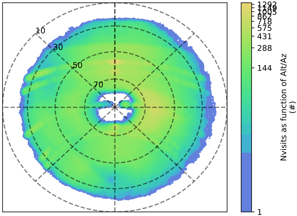
too_combined_no_gw_s10.0_v3.4_10yrs g: Nvisits as function of Alt/Az
