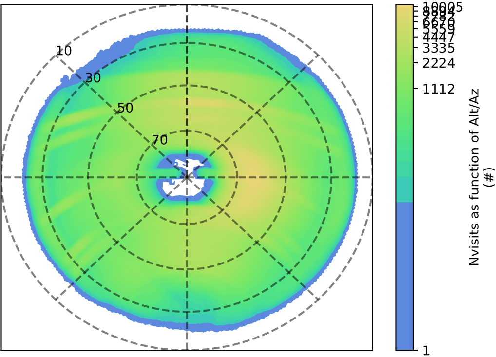
too_combined_no_gw_s10.0_v3.4_10yrs : Nvisits as function of Alt/Az
