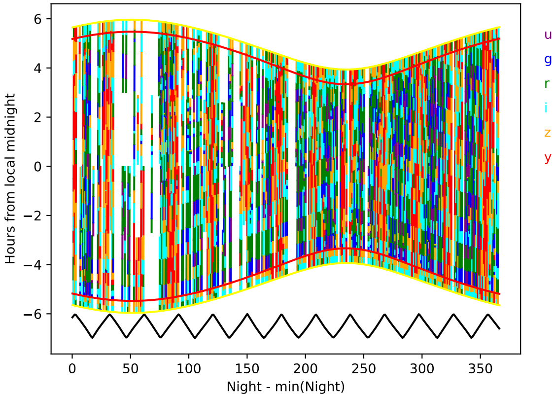
too_combined_no_gw_s10.0_v3.4_10yrs year 9-10: Hourglass
