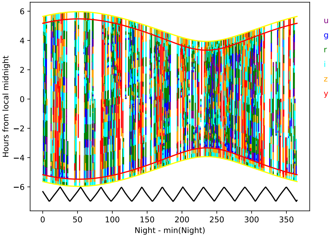
too_combined_no_gw_s10.0_v3.4_10yrs year 7-8: Hourglass
