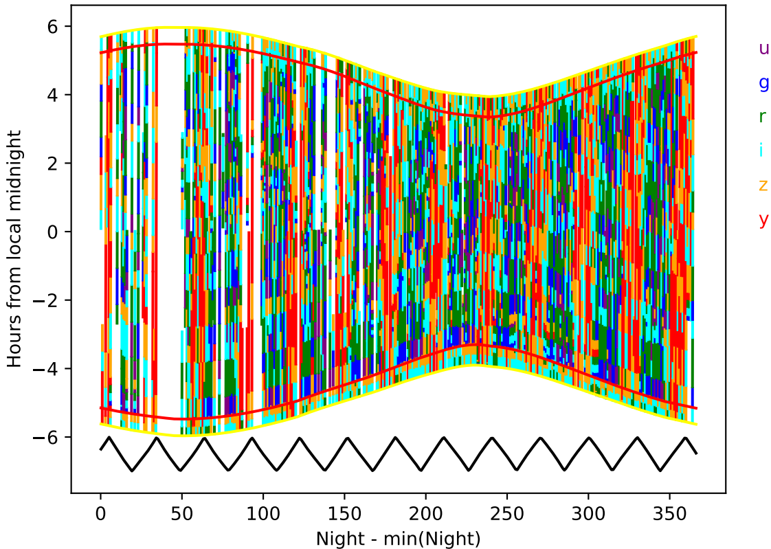
too_combined_no_gw_s10.0_v3.4_10yrs year 6-7: Hourglass
