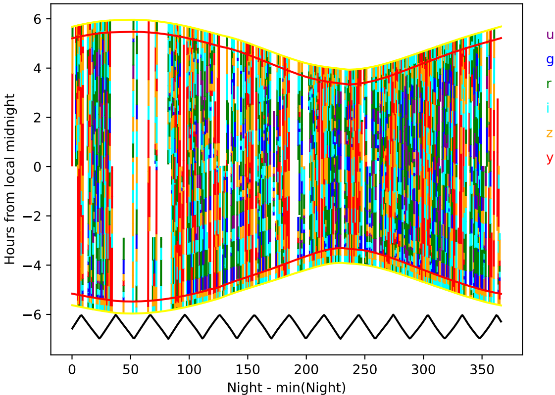
too_combined_no_gw_s10.0_v3.4_10yrs year 3-4: Hourglass
