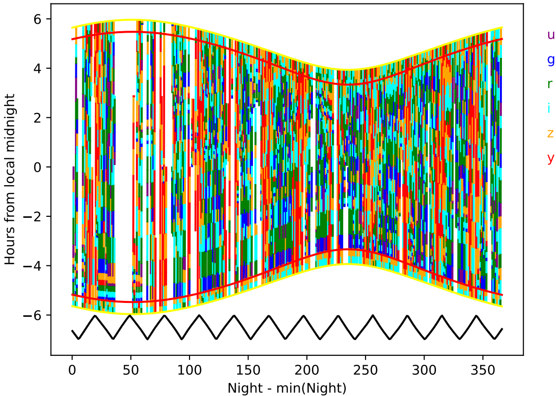
too_combined_no_gw_s10.0_v3.4_10yrs year 2-3: Hourglass
