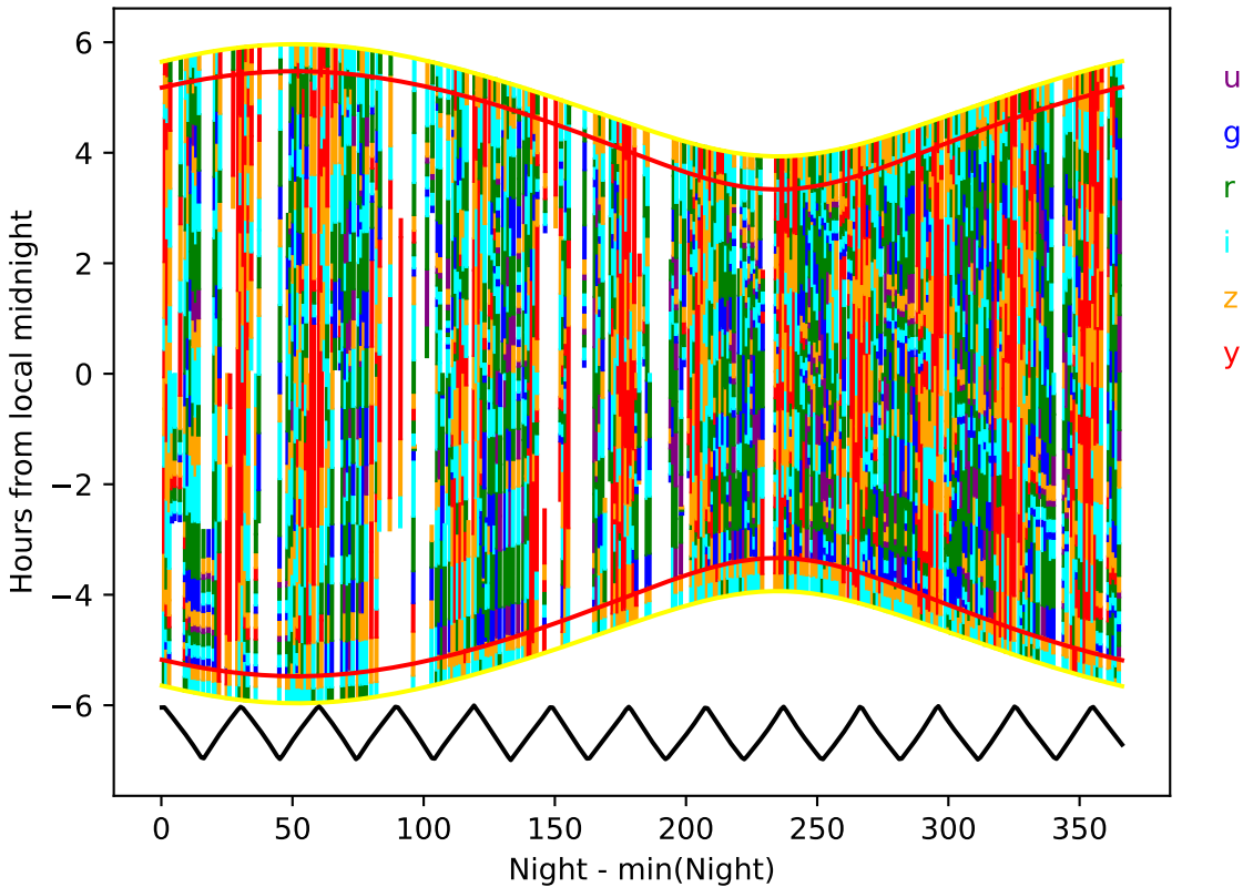
too_combined_no_gw_s10.0_v3.4_10yrs year 1-2: Hourglass
