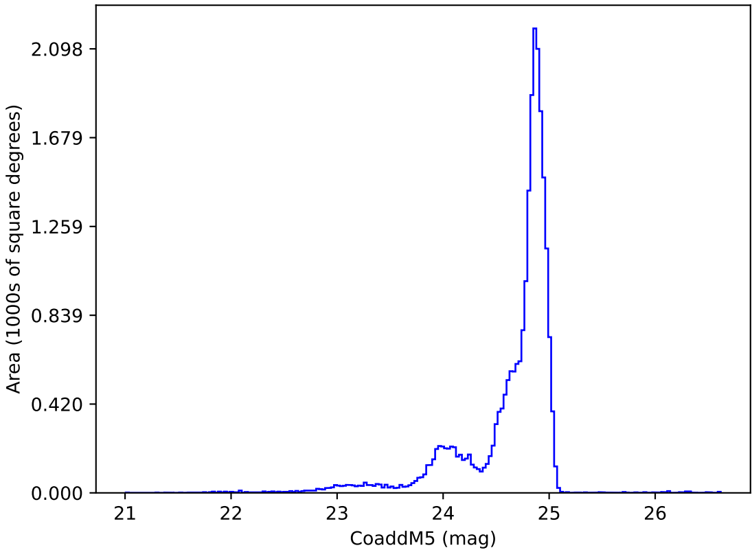
too_combined_no_gw_s10.0_v3.4_10yrs y: CoaddM5
