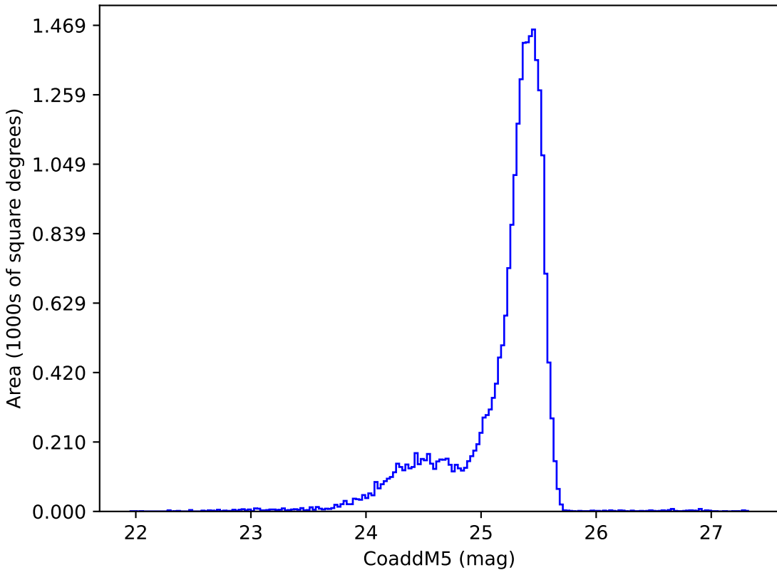
too_combined_no_gw_s10.0_v3.4_10yrs u: CoaddM5
