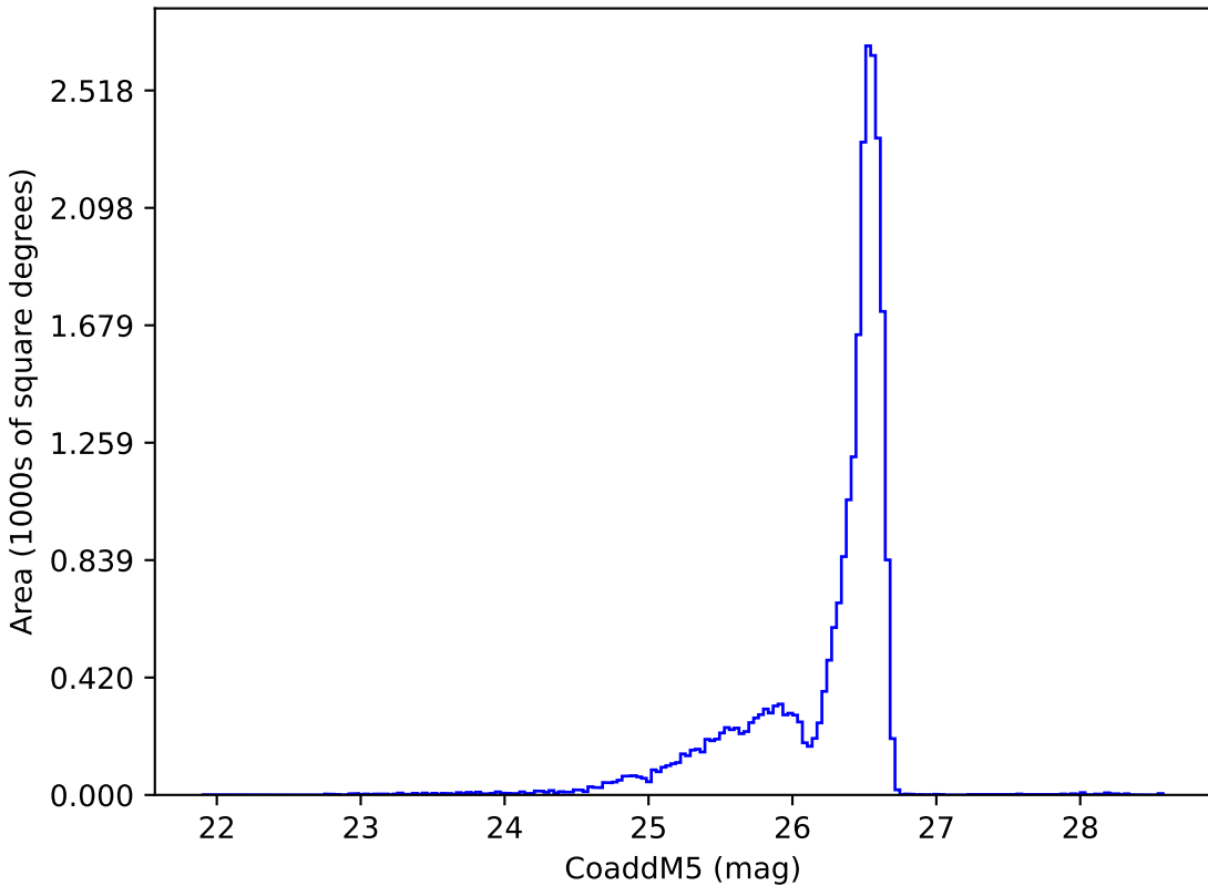
too_combined_no_gw_s10.0_v3.4_10yrs i: CoaddM5
