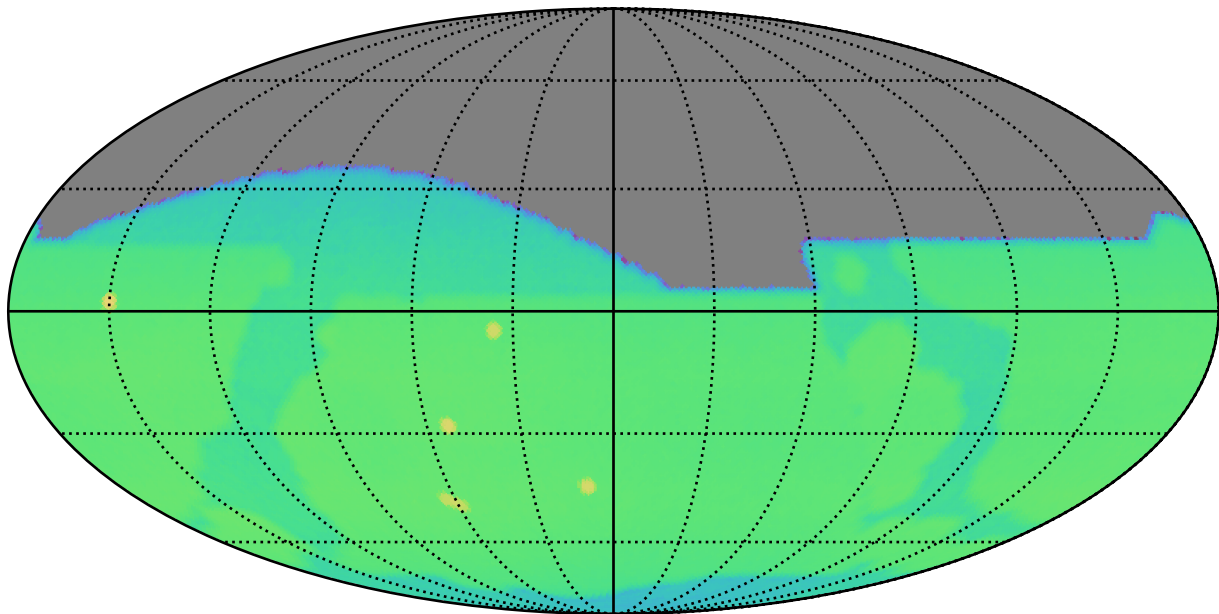
too_combined_no_gw_s10.0_v3.4_10yrs : CoaddM5
