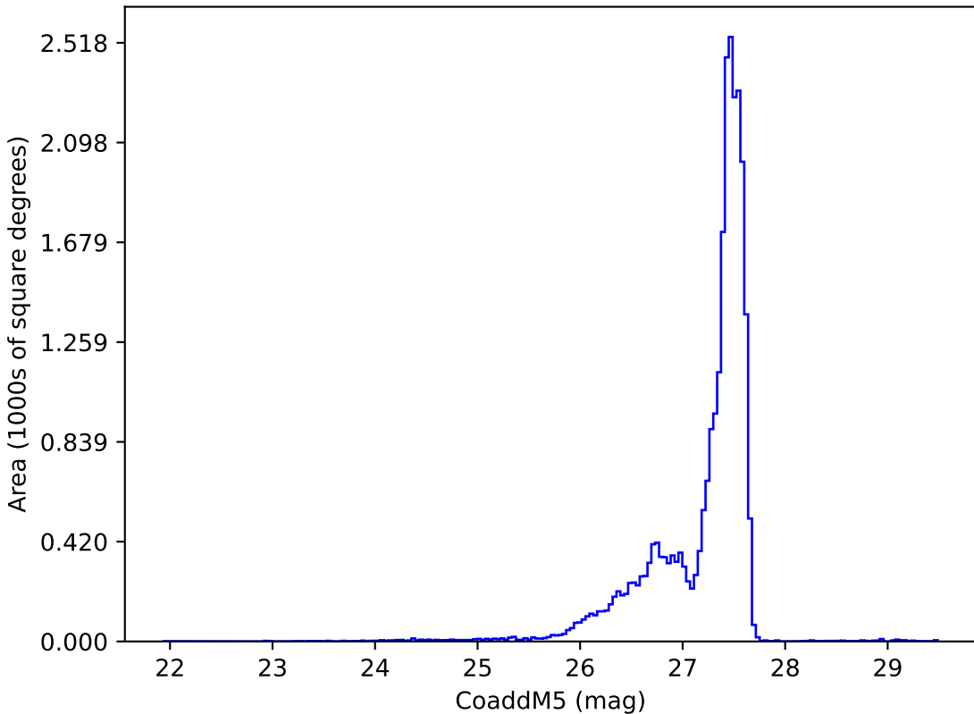
too_combined_no_gw_s10.0_v3.4_10yrs : CoaddM5
