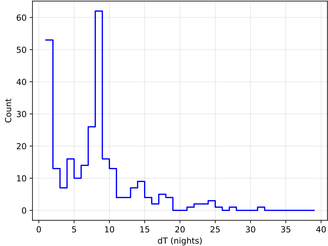
too_combined_no_gw_s10.0_v3.4_10yrs all bands: DD:XMM_LSS Delta Nights Histogram
