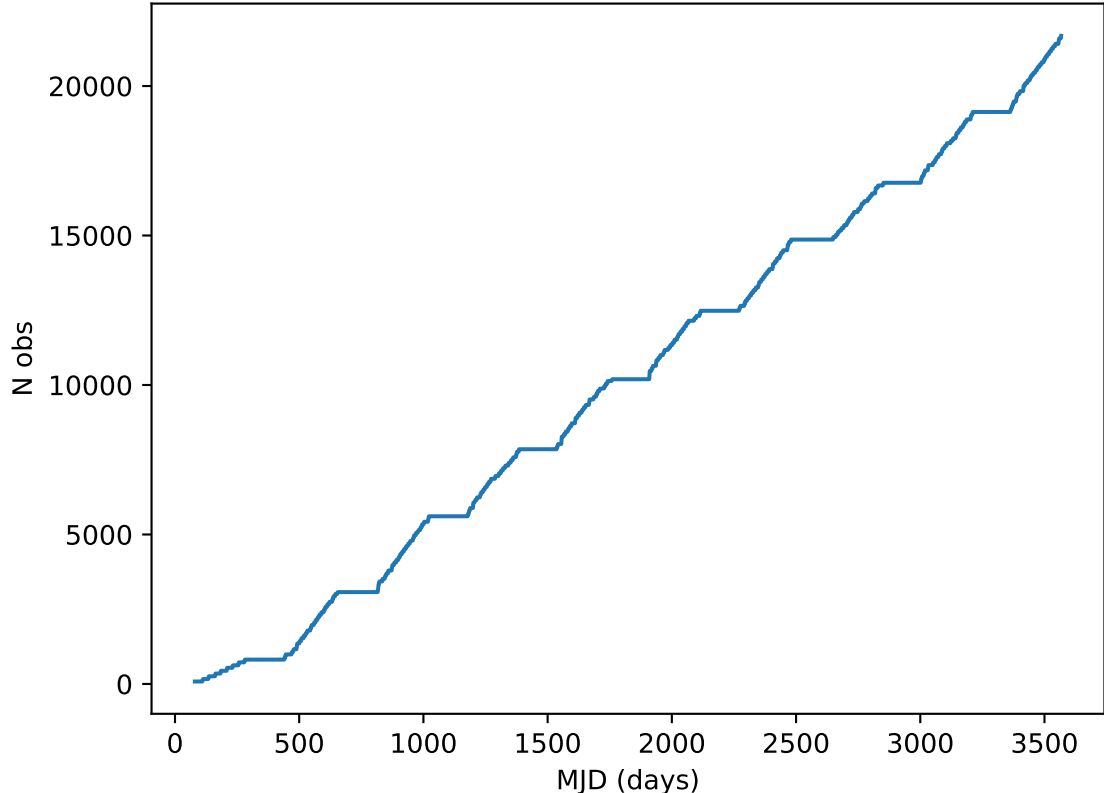
too_combined_no_gw_s10.0_v3.4_10yrs all bands: DD:XMM_LSS Cumulative NVisits
