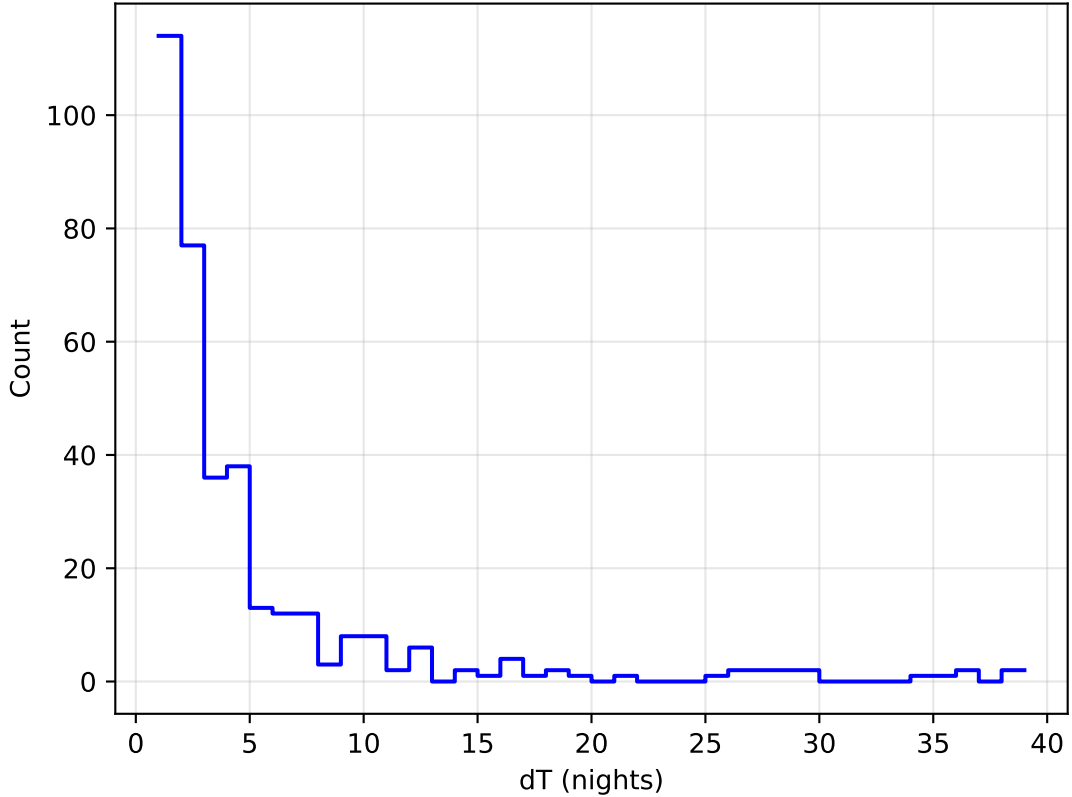
too_combined_no_gw_s10.0_v3.4_10yrs all bands: DD:WFD Delta Nights Histogram
