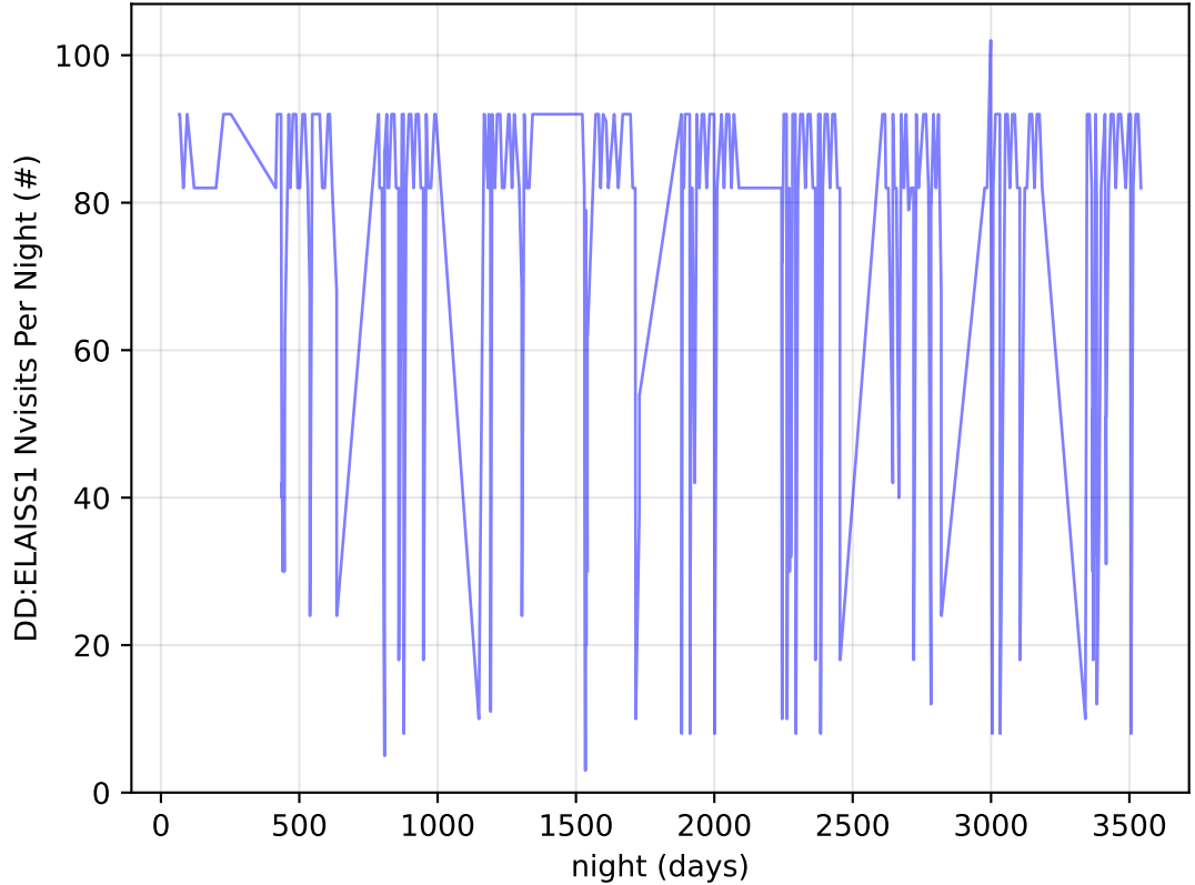
too_combined_no_gw_s10.0_v3.4_10yrs all bands: DD:ELAISS1 Nvisits Per Night
