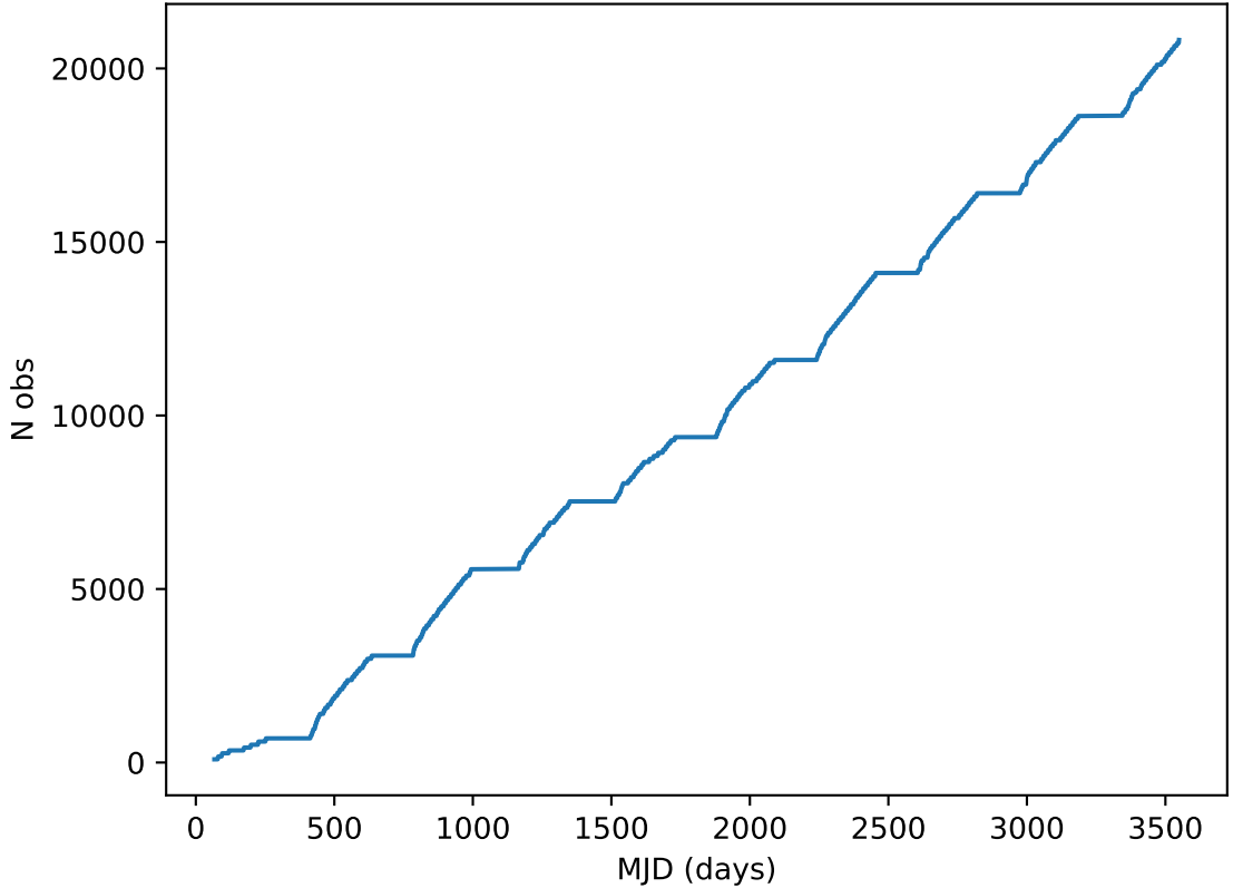
too_combined_no_gw_s10.0_v3.4_10yrs all bands: DD:ELAISS1 Cumulative NVisits
