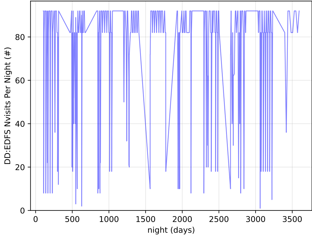
too_combined_no_gw_s10.0_v3.4_10yrs all bands: DD:EDFS Nvisits Per Night
