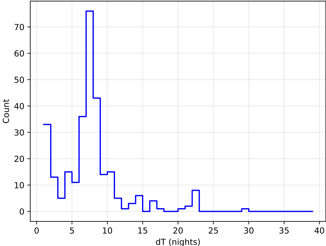
too_combined_no_gw_s10.0_v3.4_10yrs all bands: DD:EDFS Delta Nights Histogram
