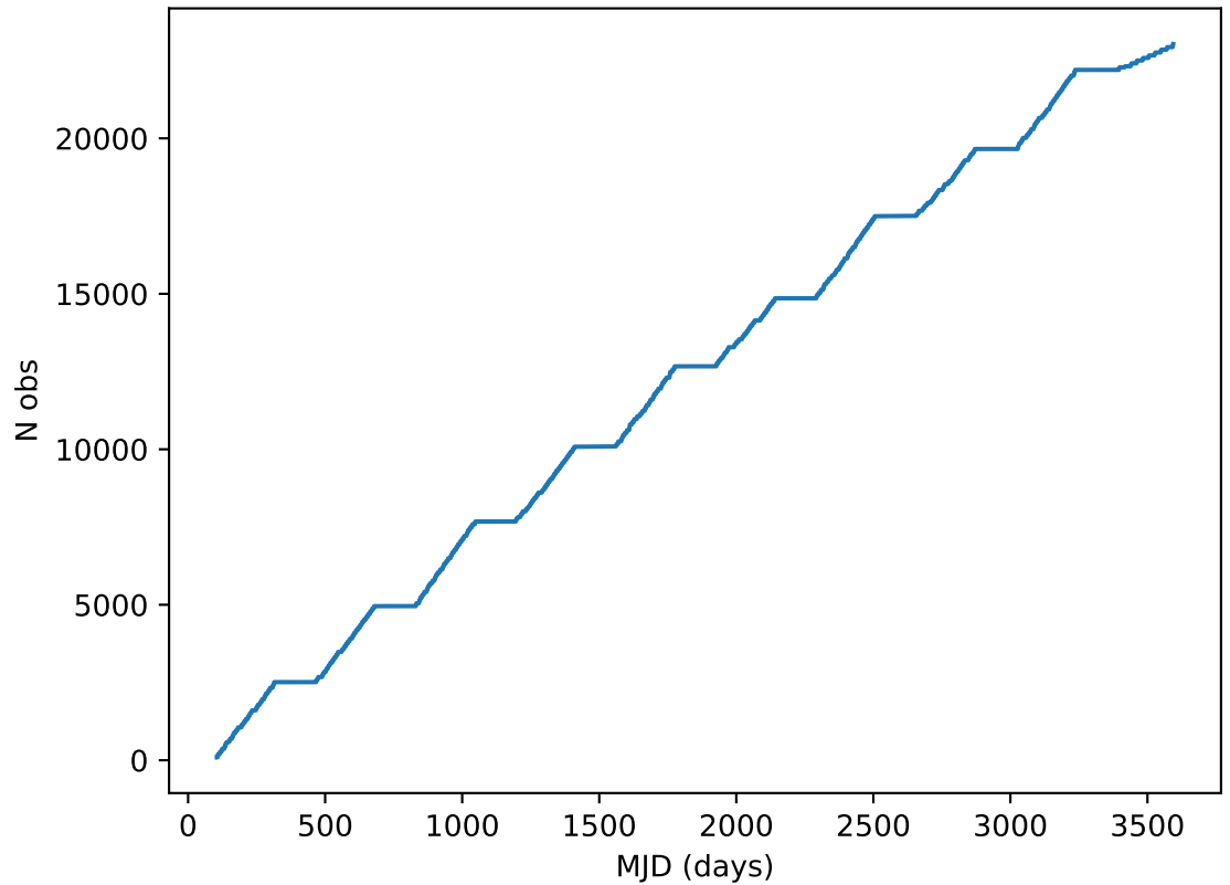
too_combined_no_gw_s10.0_v3.4_10yrs all bands: DD:EDFS Cumulative NVisits
