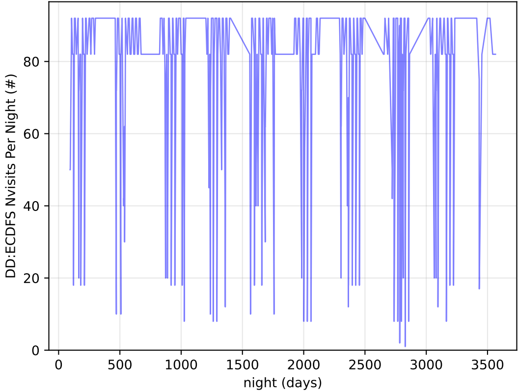
too_combined_no_gw_s10.0_v3.4_10yrs all bands: DD:ECDFS Nvisits Per Night
