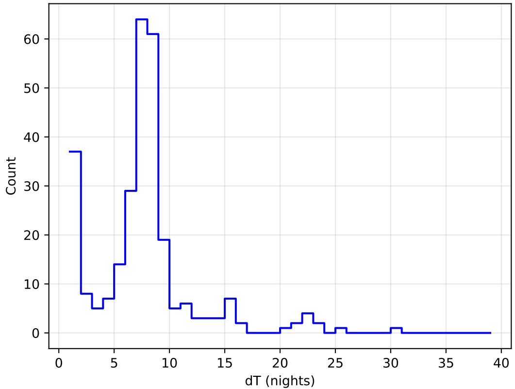
too_combined_no_gw_s10.0_v3.4_10yrs all bands: DD:ECDFS Delta Nights Histogram
