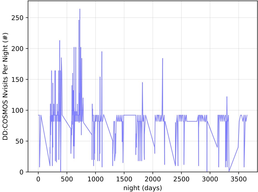
too_combined_no_gw_s10.0_v3.4_10yrs all bands: DD:COSMOS Nvisits Per Night
