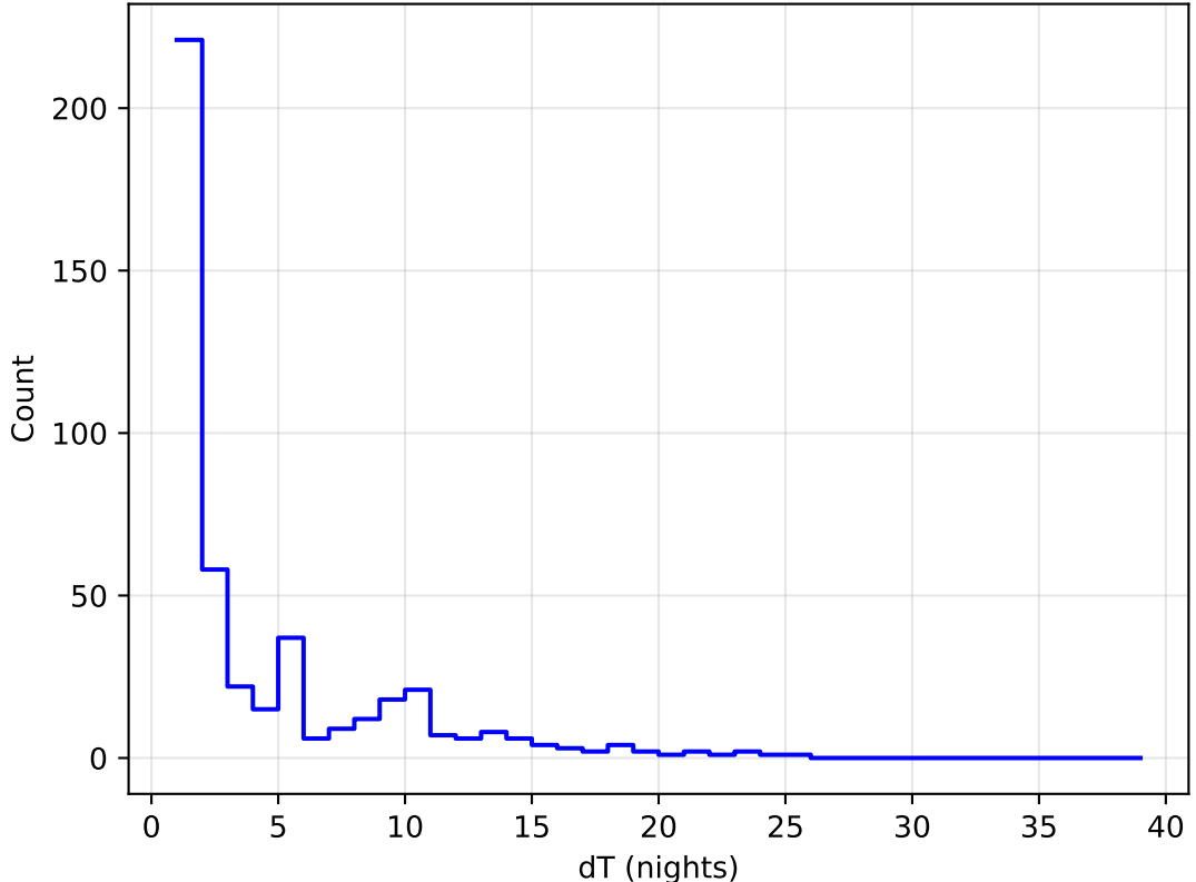
too_combined_no_gw_s10.0_v3.4_10yrs all bands: DD: COSMOS Delta Nights Histogram
