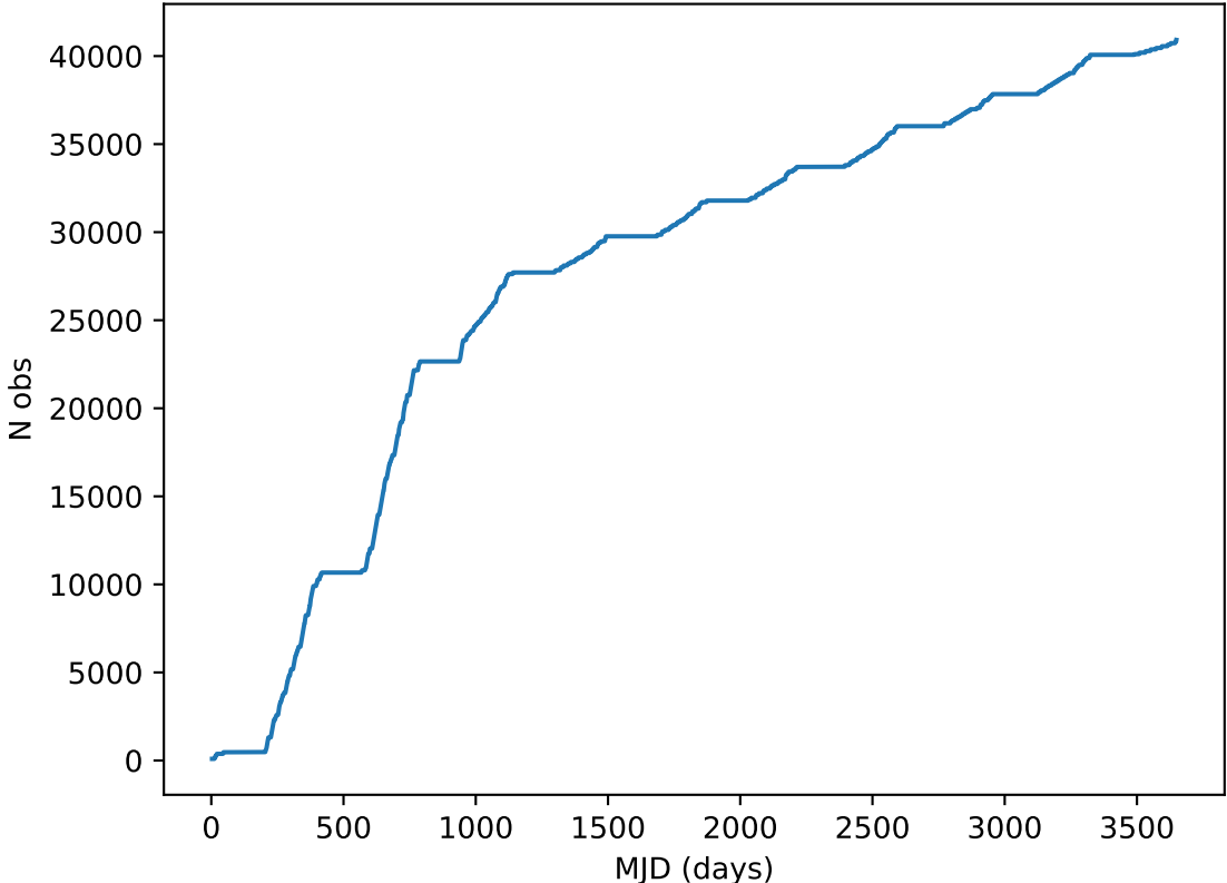
too_combined_no_gw_s10.0_v3.4_10yrs all bands: DD:COSMOS Cumulative NVisits
