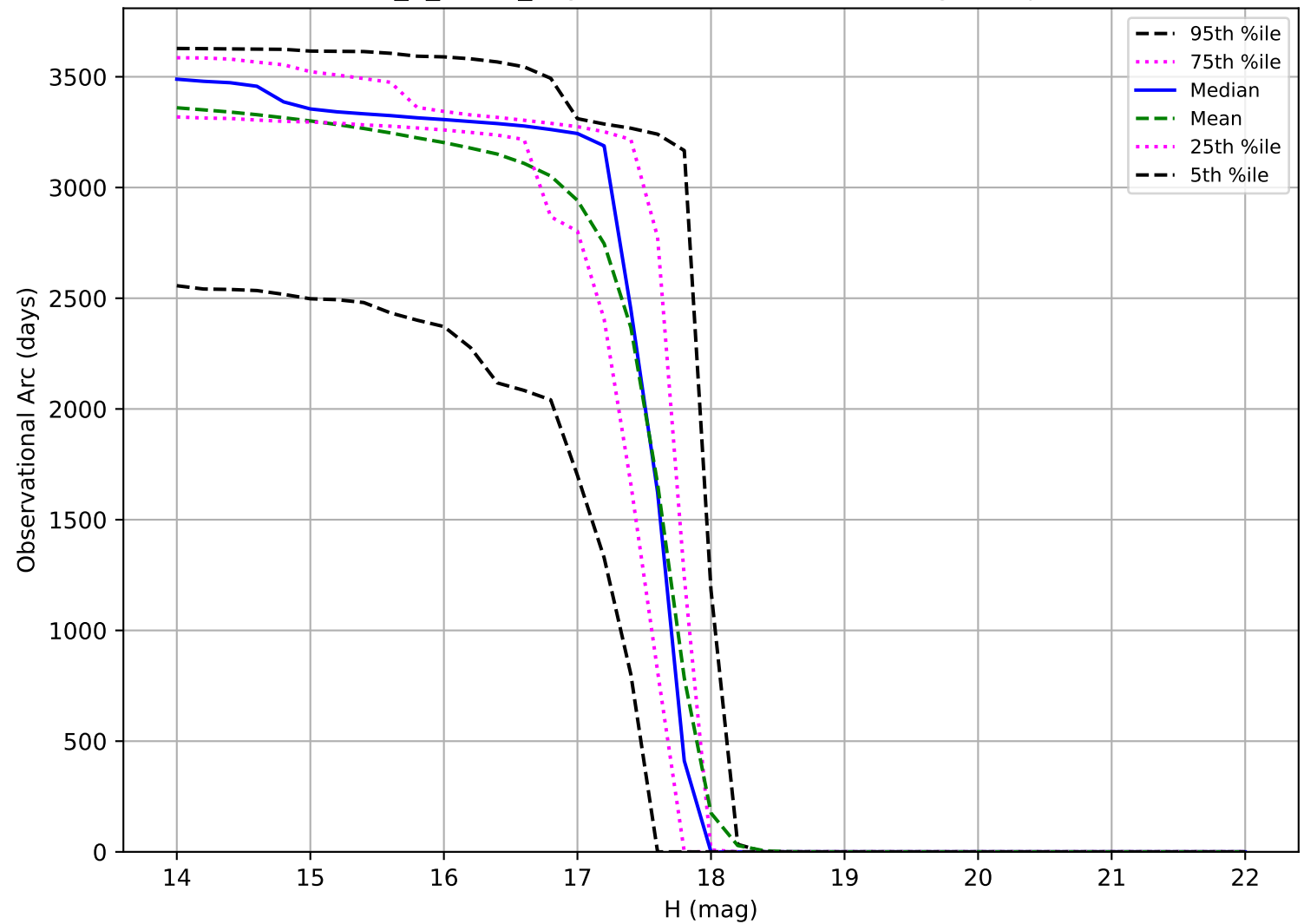
too_5_4v3.4_10yrs: Observational Arc Length Trojan
