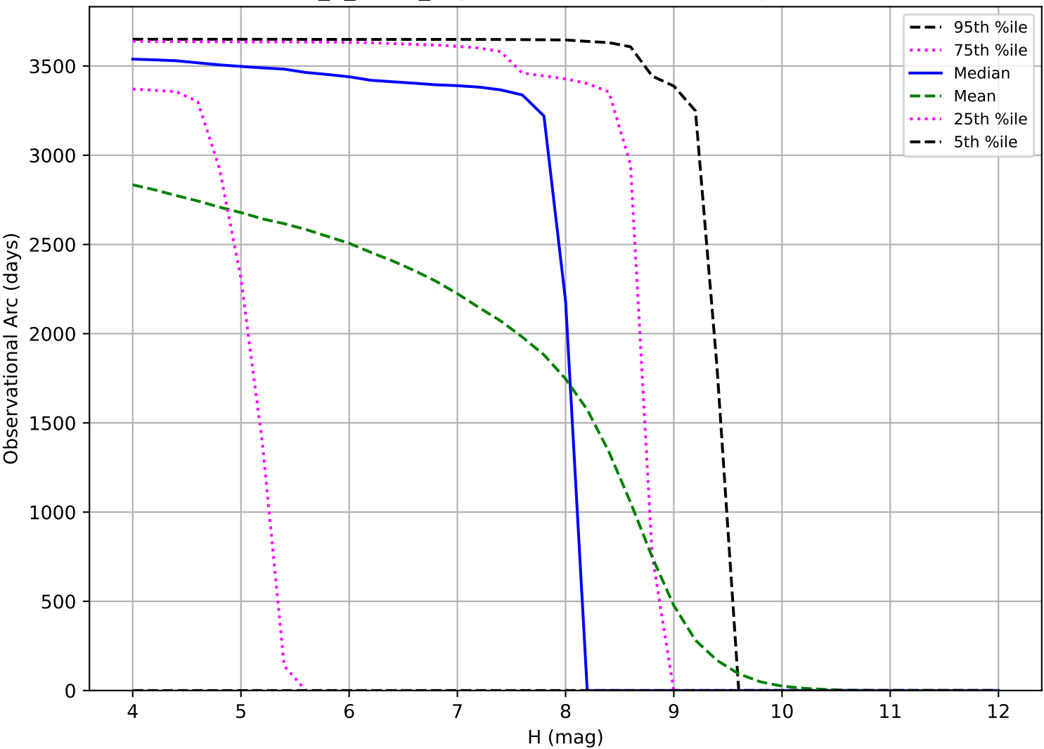
too_5_4v3.4_10yrs: Observational Arc Length TNO
