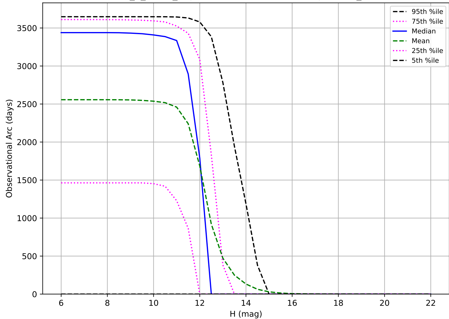
too_5_4v3.4_10yrs: Observational Arc Length OCC_r20
