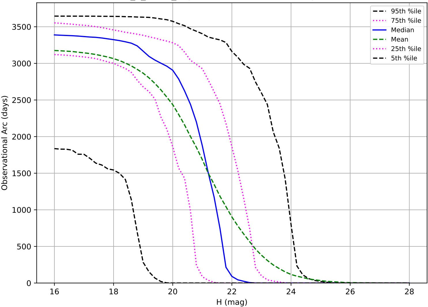
too_5_4v3.4_10yrs: Observational Arc Length NEO
