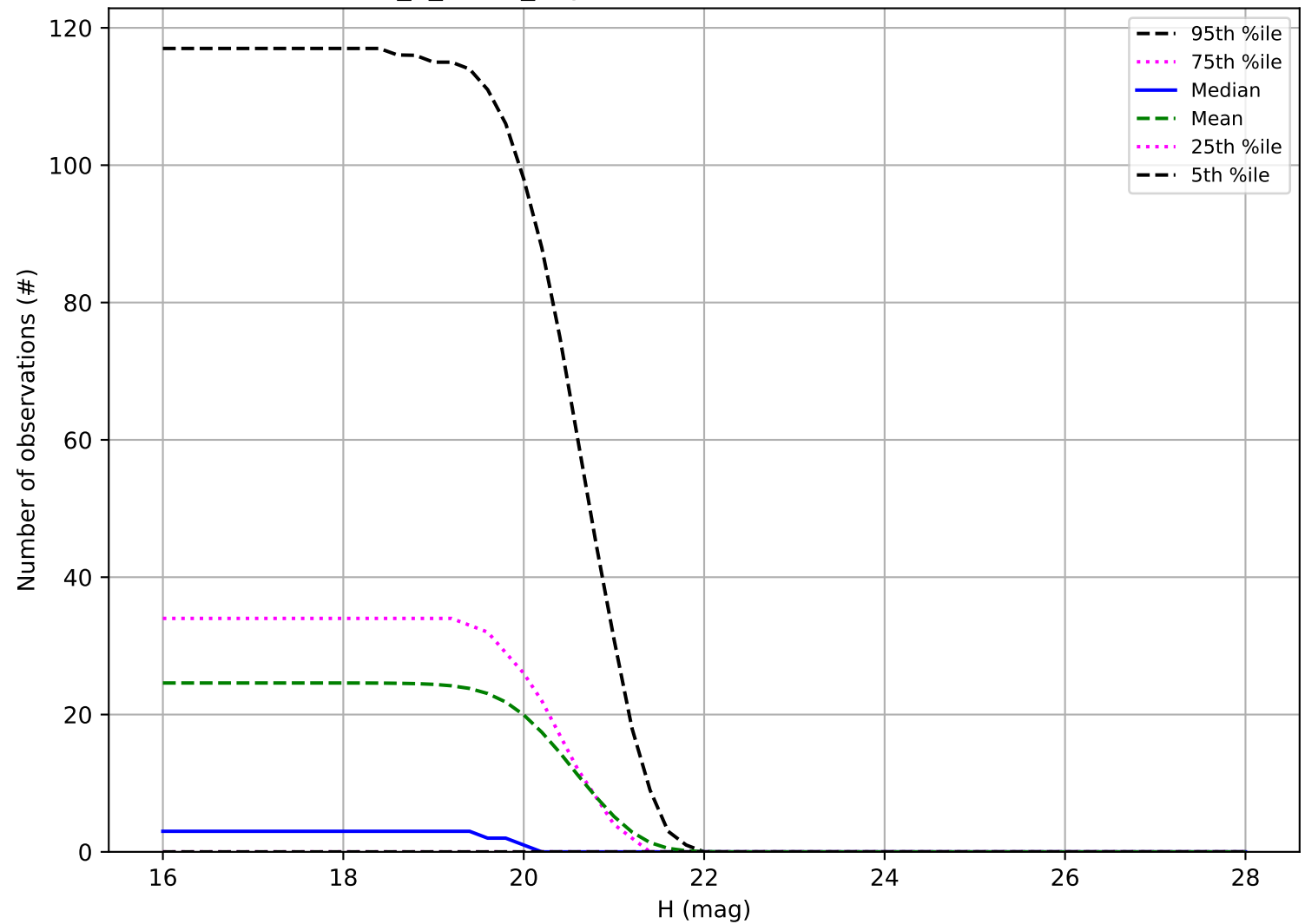
too_5_4v3.4_10yrs: Number of observations Vatira
