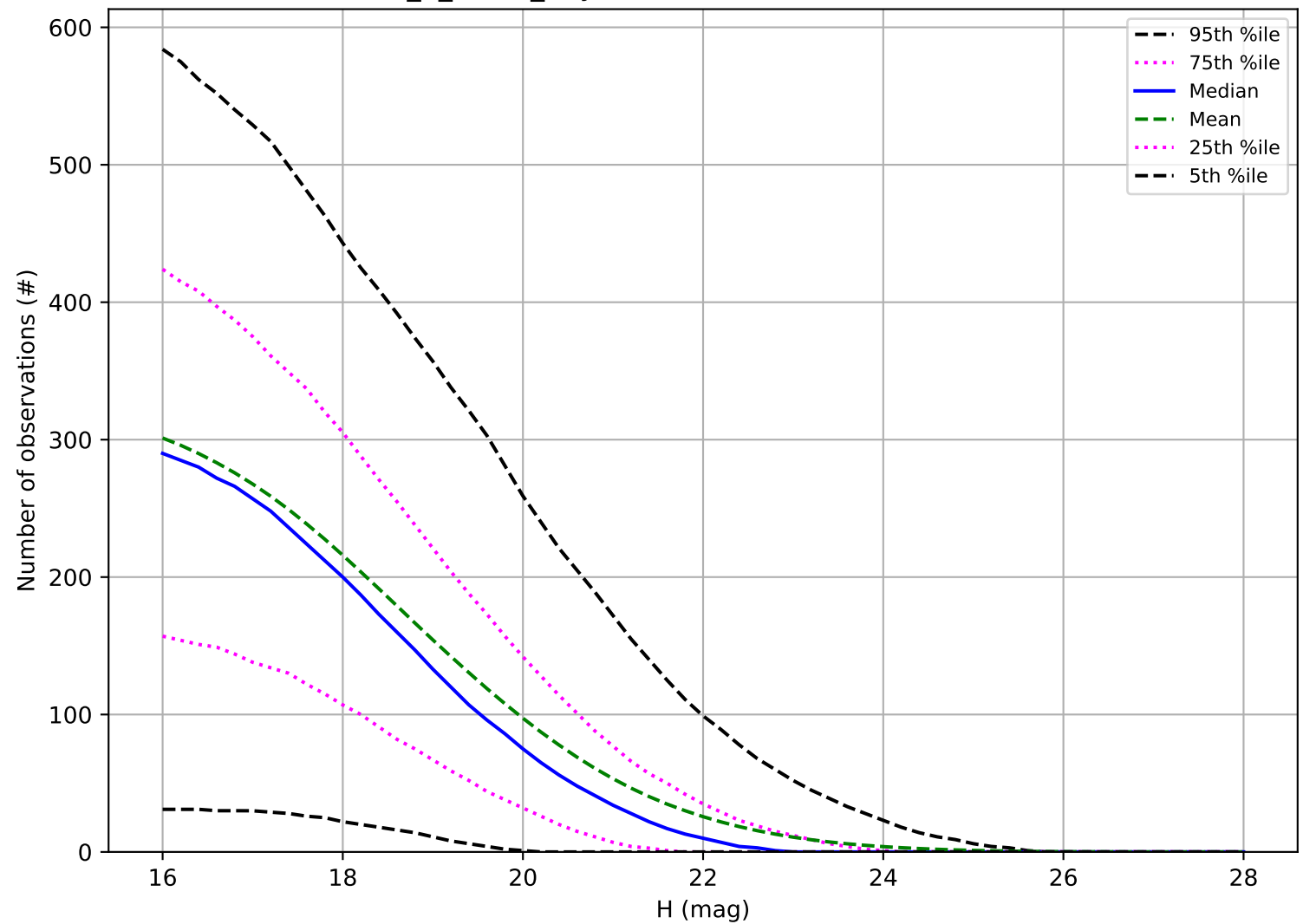
too_5_4v3.4_10yrs: Number of observations NEO
