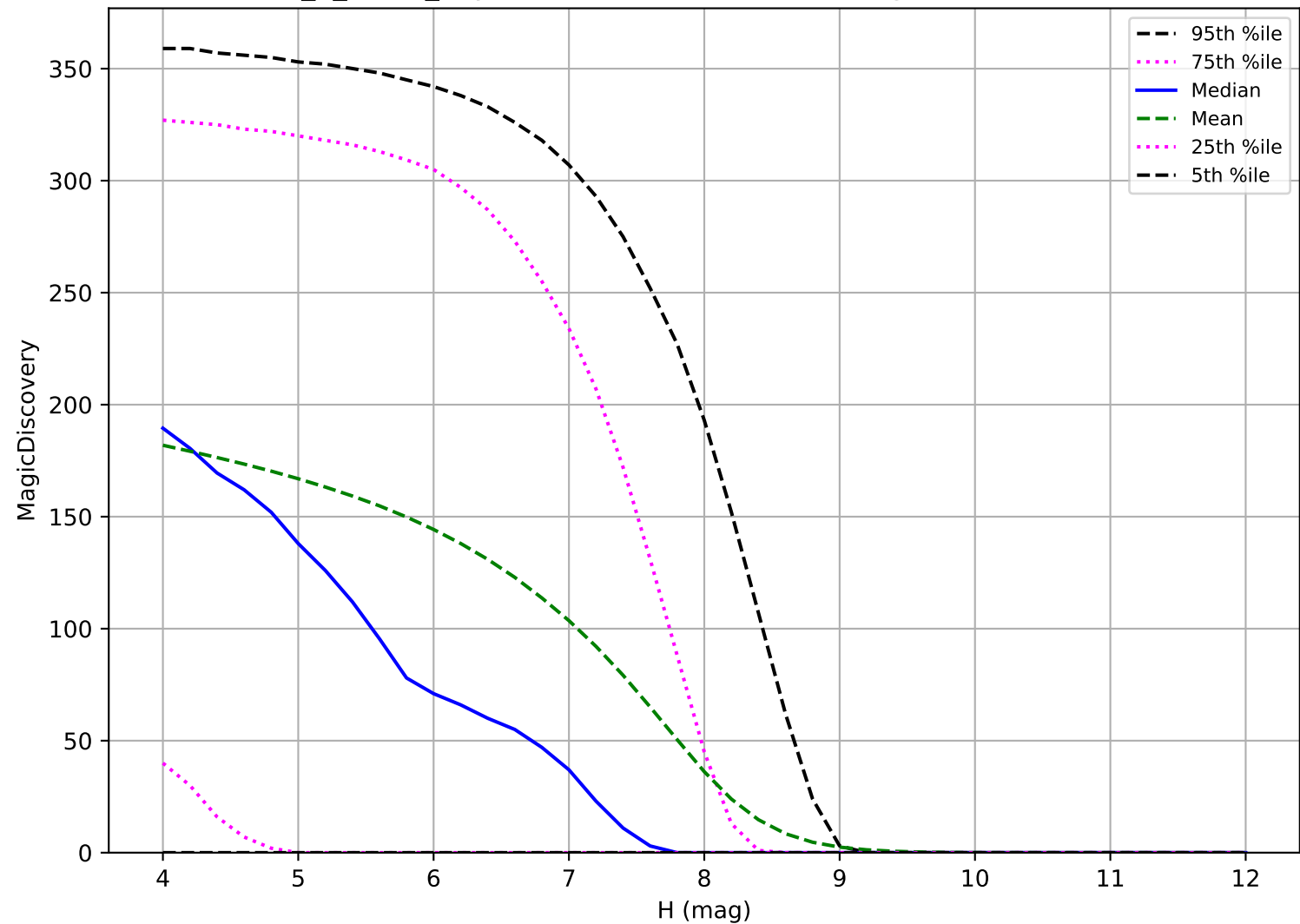
too_5_4v3.4_10yrs: TNO 6 detections in 60 nights detection loss
