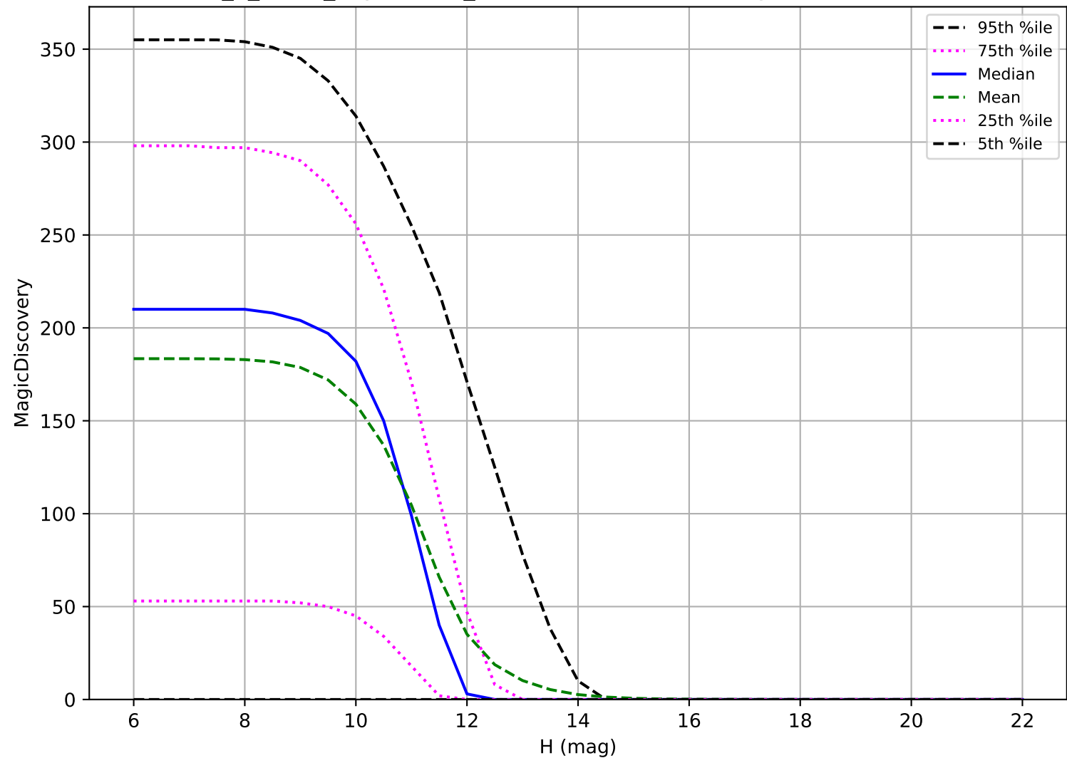
too_5_4v3.4_10yrs: OCC_r20 6 detections in 60 nights detection loss
