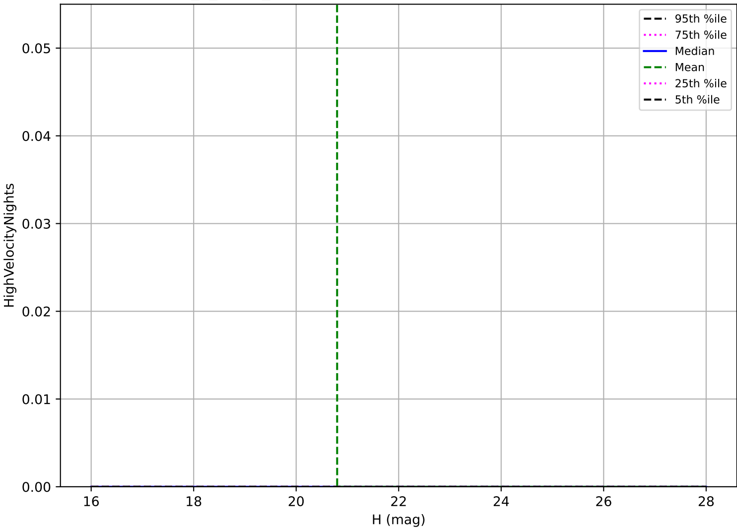
too_5_4v3.4_10yrs: Vatira High velocity pair detection loss
