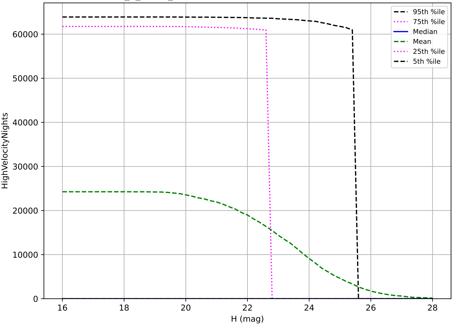
too_5_4v3.4_10yrs: PHA High velocity pair detection loss
