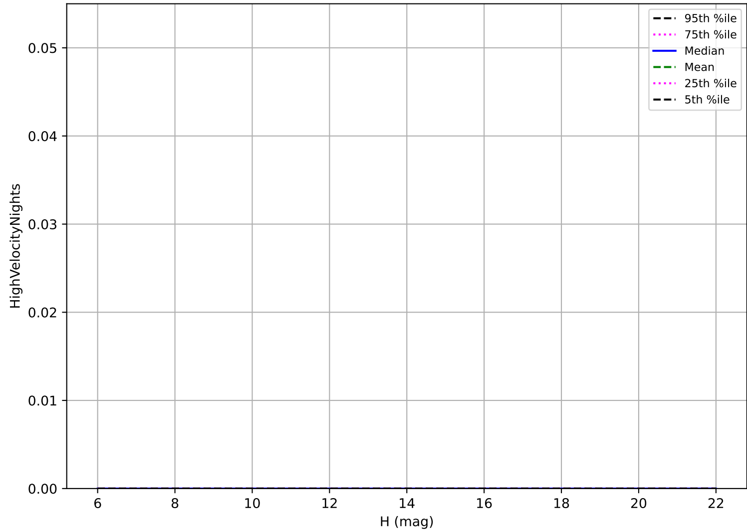
too_5_4v3.4_10yrs: OCC_r5 High velocity pair detection loss
