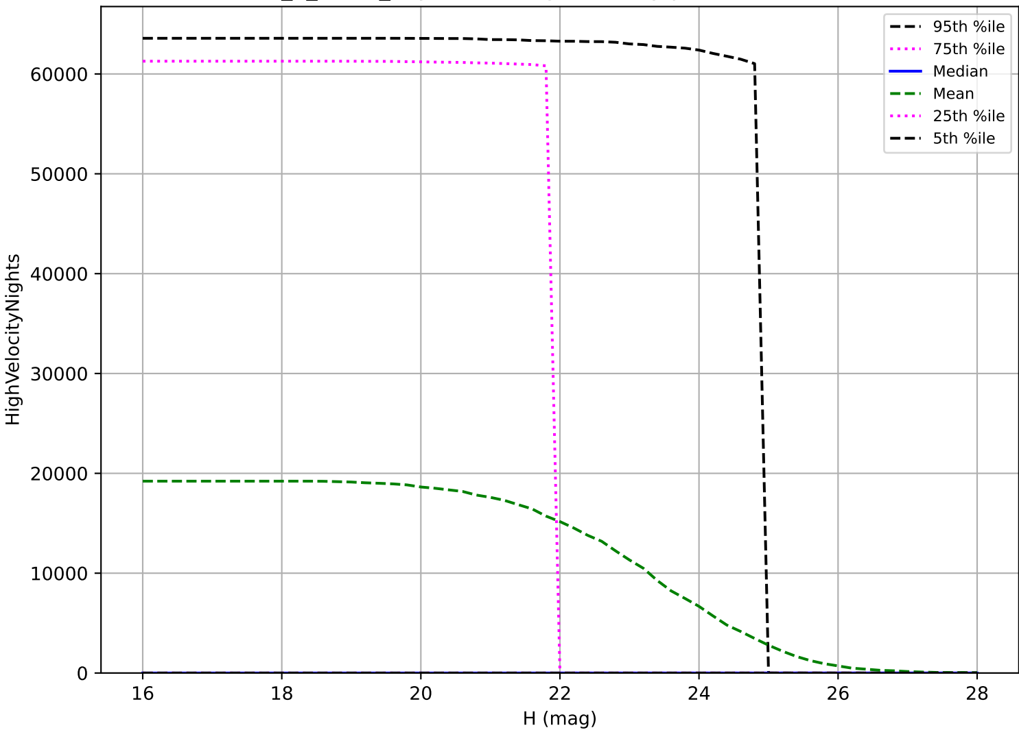
too_5_4v3.4_10yrs: NEO High velocity pair detection loss
