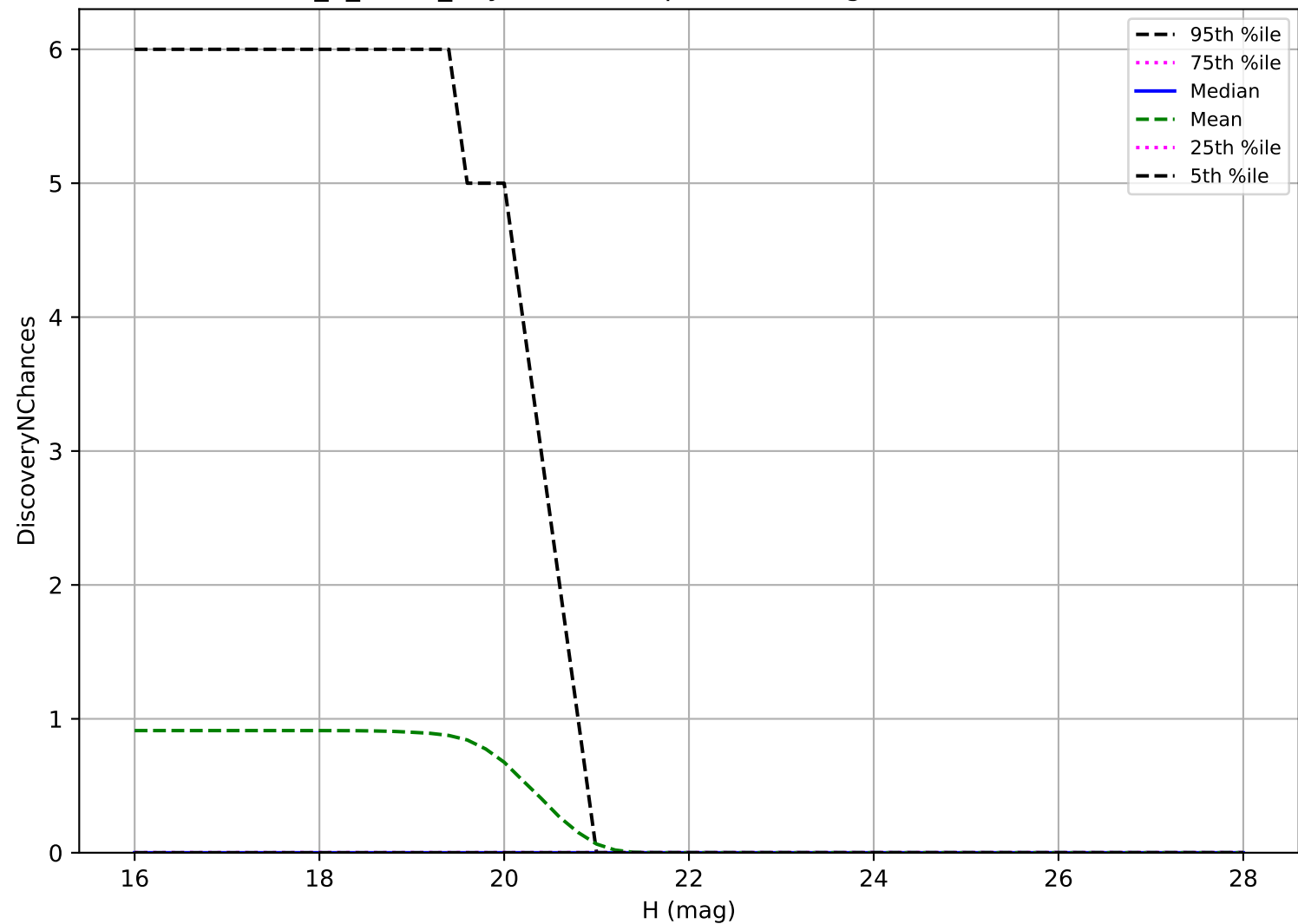
too_5_4v3.4_10yrs: Vatira 3 pairs in 15 nights detection loss
