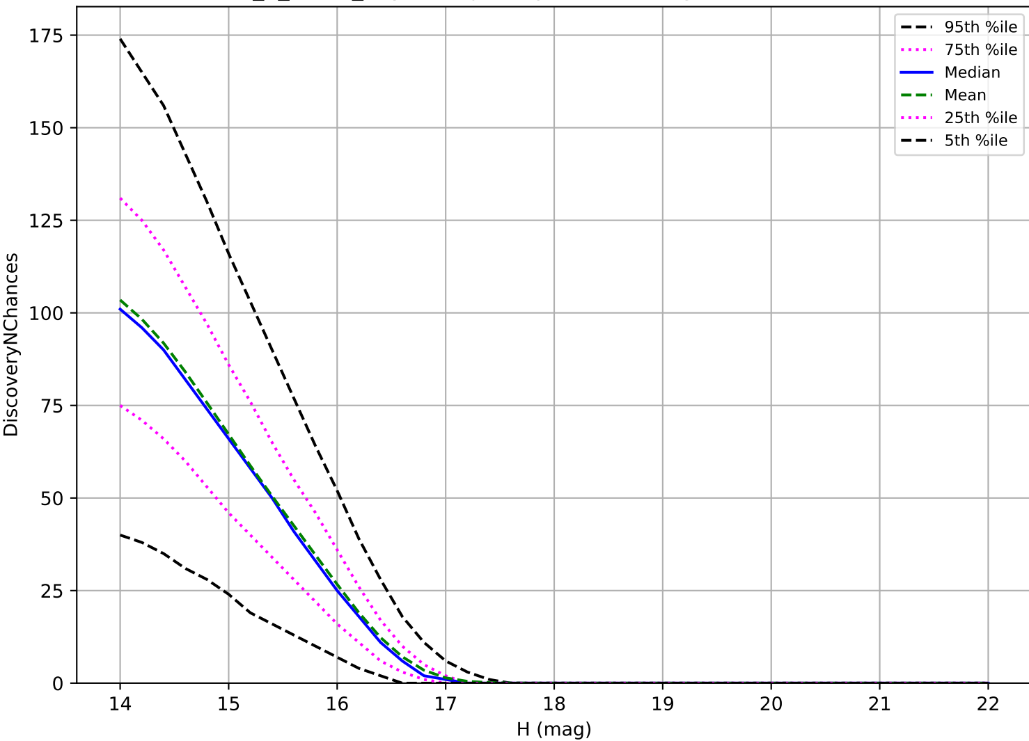
too_5_4v3.4_10yrs: Trojan 3 pairs in 15 nights detection loss
