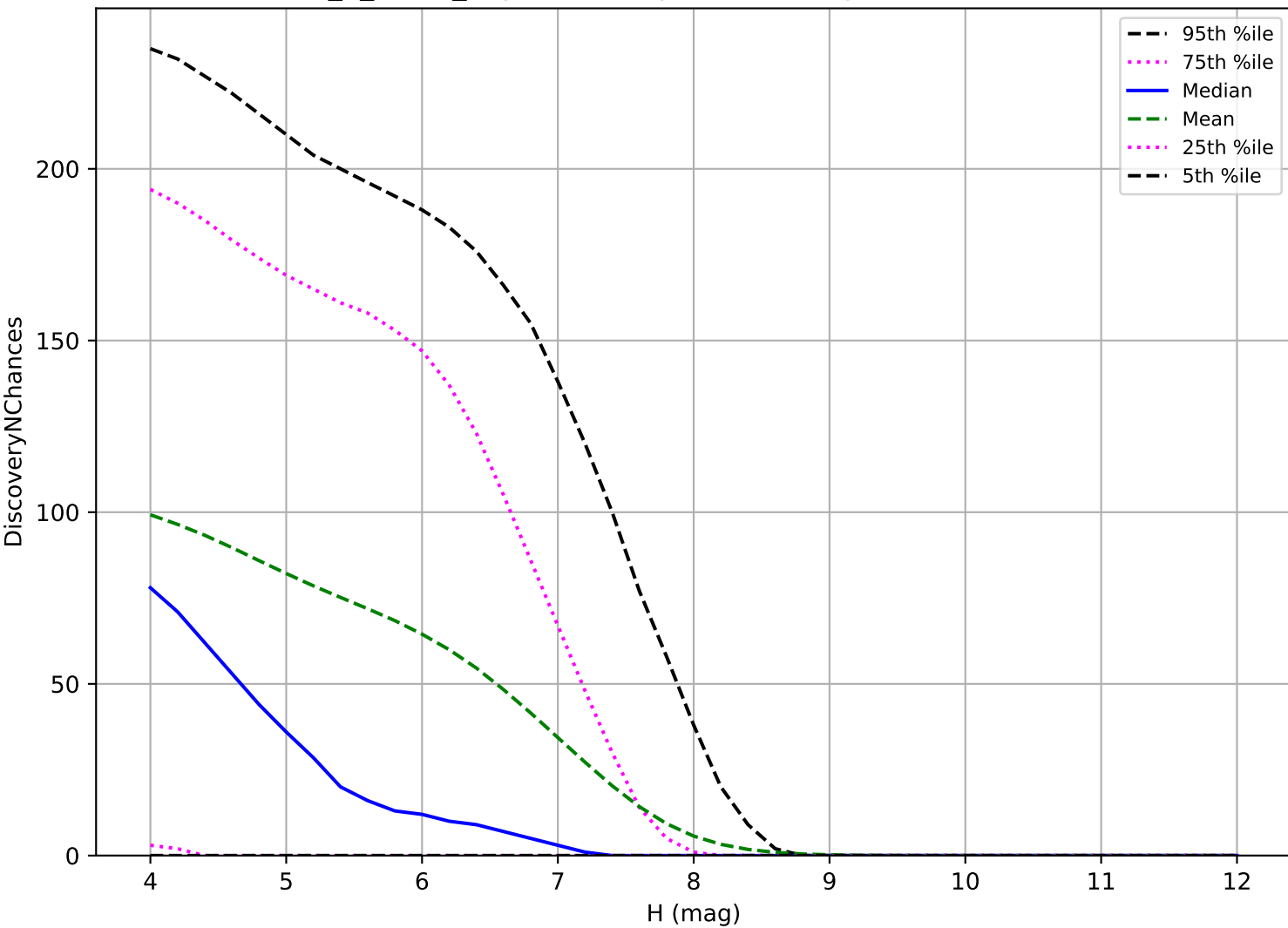
too_5_4v3.4_10yrs: TNO 3 pairs in 15 nights detection loss
